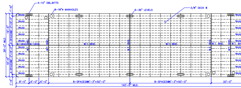
DECK PLAN
