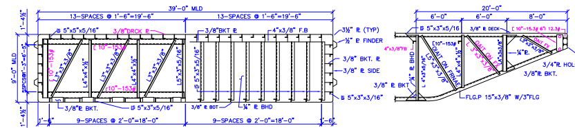
TYPICAL TRANSV. TRUSS
